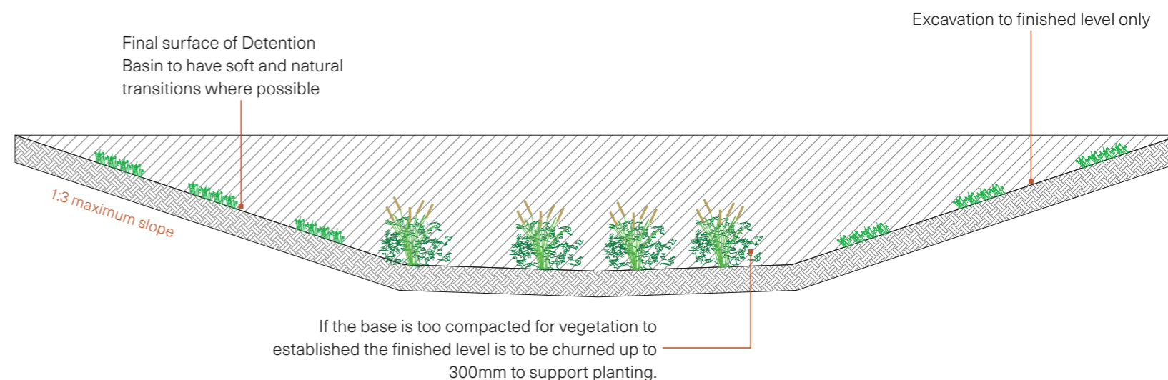
Figure 15: Typical Detention Basin Detail
